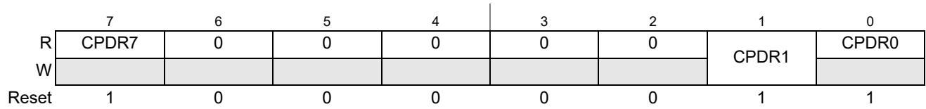
Figure 17-2. Port CP Data Register (CPDR)
