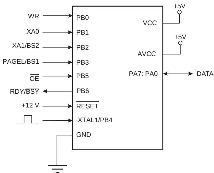
Figure 58. Parallel Programming
