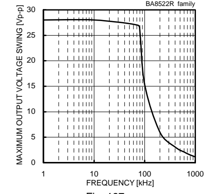
Fig. 197 Maximum Output Voltage Swing - Frequency (VCC/VEE=+15[V]/-15[V], RL=2[kΩ], Ta=25[°C])
