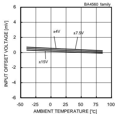
Fig. 54 Input Offset Voltage - Ambient Temperature (Vicm=0[V], Vout=0[V])
