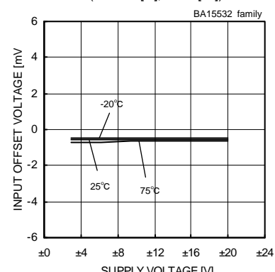
Fig. 251 Input Offset Voltage - Supply Voltage (Vicm=0[V], Vout=0[V])
