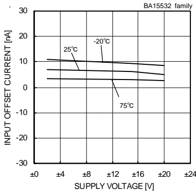
Fig. 255 Input Offset Current - Supply Voltage ( V_{icm}=0[V] , V_{out}=0[V] )
