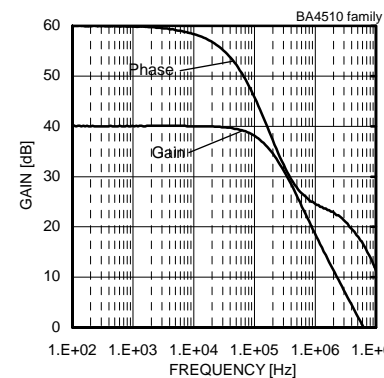
Fig. 287 Voltage Gain - Frequency (V CC /V EE =2.5[V]/-2.5[V], A v =40[dB], R L =10[kΩ])
