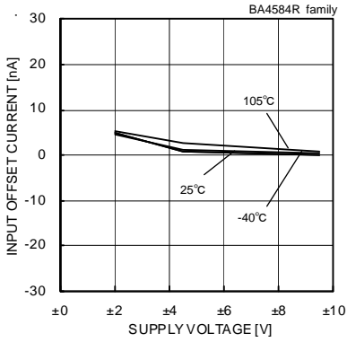
Fig. 167 Input Offset Current - Supply Voltage (V icm =0[V], V out =0[V])
