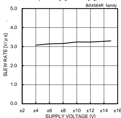
Fig. 106 Slew Rate - Supply Voltage ( C_L=100[pF] , R_L=2[kΩ] , T_a=25[°C] )
