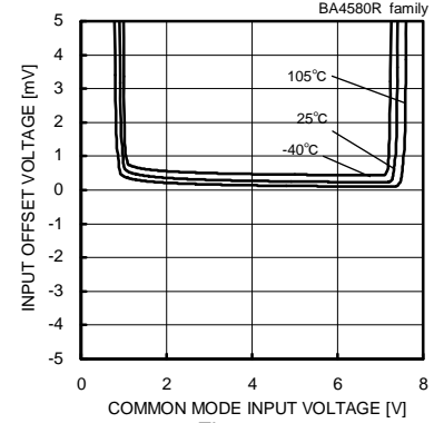
Fig. 125 Input Offset Voltage - Common Mode Input Voltage ( V_{CC}=8[V] , V_{out}=4[V] )
