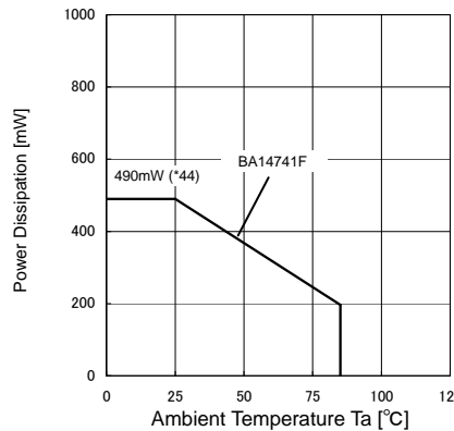
(f)BA14741F
