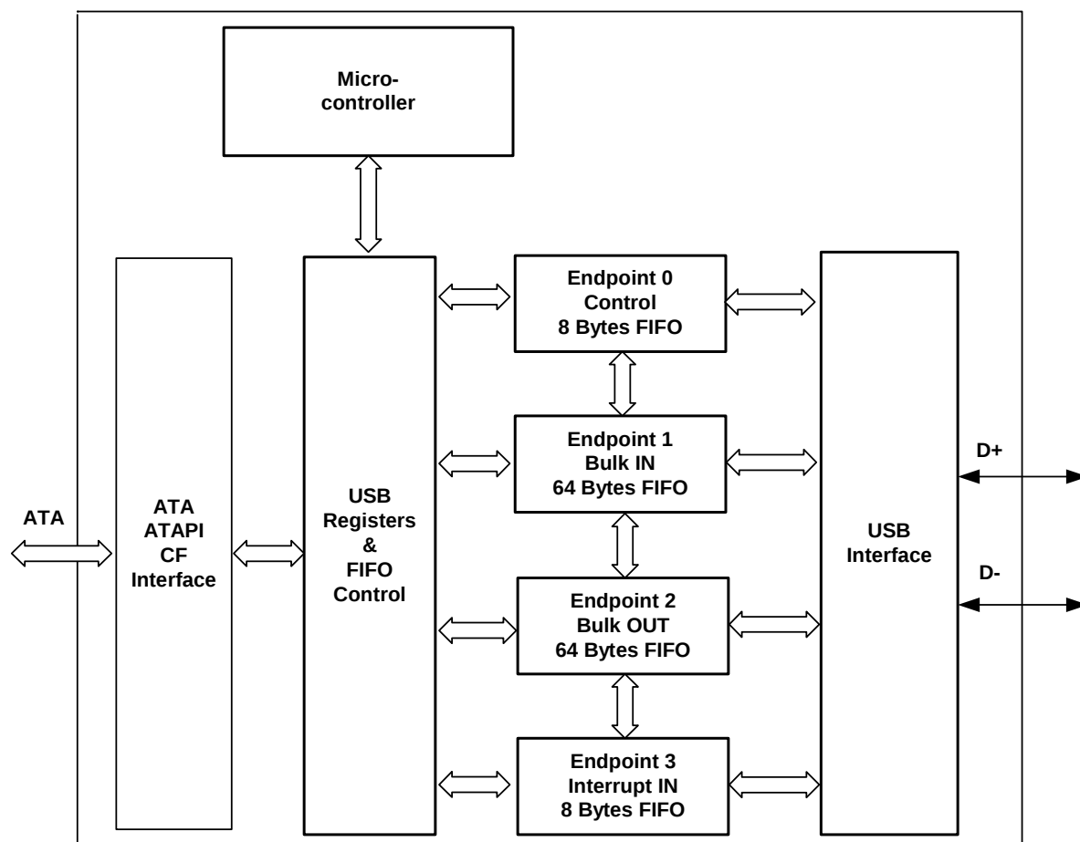
Figure 2-1 Block Diagram of GL641USB
