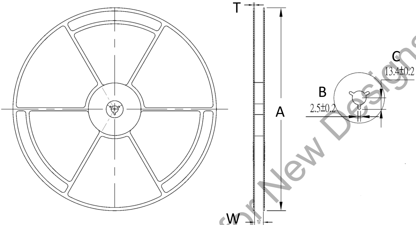
Figure 14 - Reel Specifications
