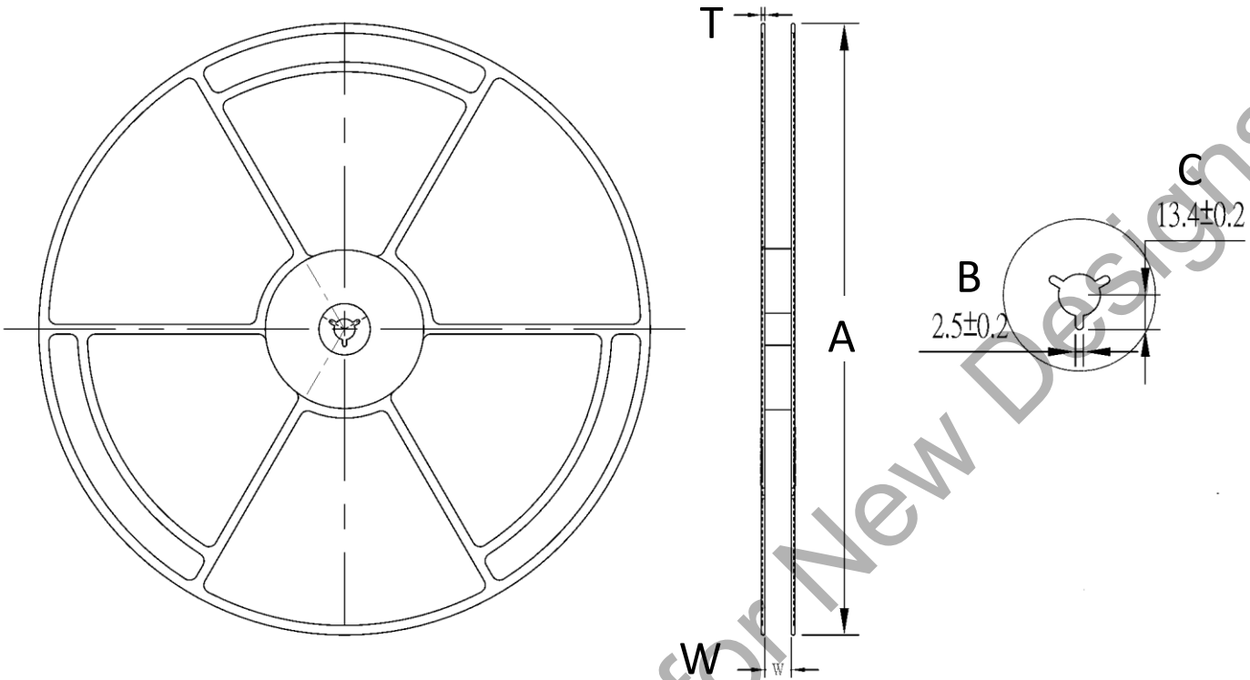
Figure 14 - Reel Specifications
