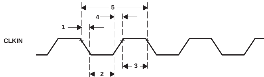
Figure 14. CLKIN Timing
