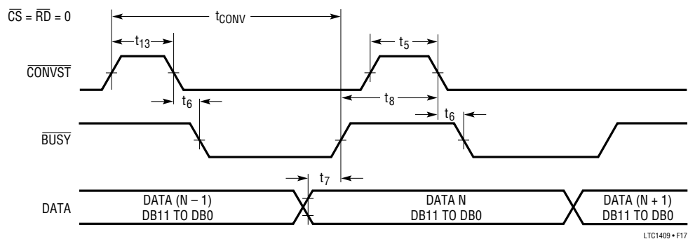
Figure 17. Mode 1b. \overline{\text{CONVST}} Starts a Conversion. Data Outputs Always Enabled
