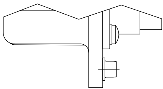
#4-40 CLINCH NUT DETAIL IN 4 CORNERS 443197-3 ONLY
