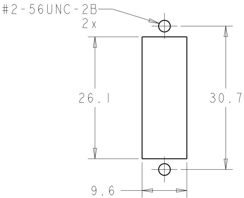
SCALE 2:1 SUGGESTED PANEL CUTOUT MAX PANEL THICKNESS 1.7
