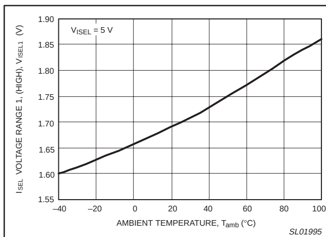
Figure 20. I_{SEL} voltage range 1 versus ambient temperature.
