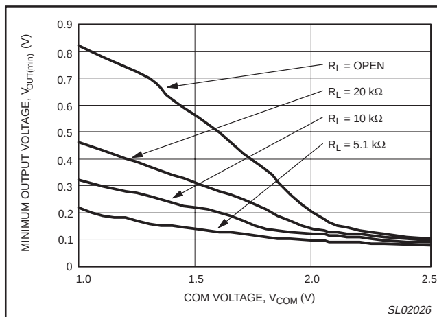
Figure 32. Minimum output voltage versus COM voltage.
