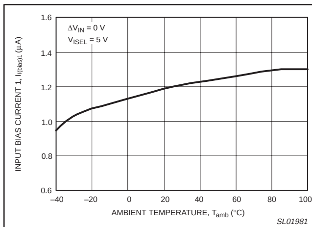
Figure 10. Input bias current versus ambient temperature.
