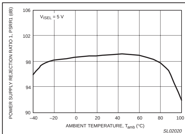
Figure 26. Power supply rejection ratio 1 versus ambient temperature.
