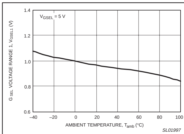
Figure 22. G_{SEL} voltage range 1 versus ambient temperature.
