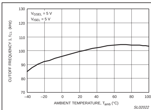
Figure 28. Cutoff frequency 1 versus ambient temperature.
