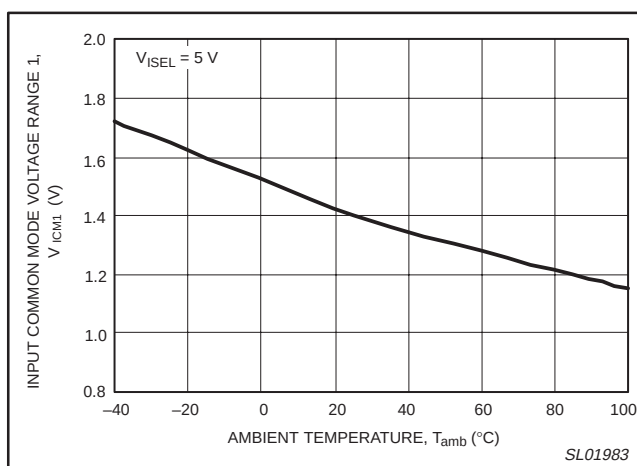
Figure 12. Input common mode voltage (minimum) versus ambient temperature.
