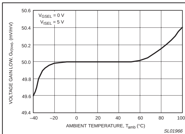
Figure 6. Voltage Gain 2 (LOW) versus ambient temperature.
