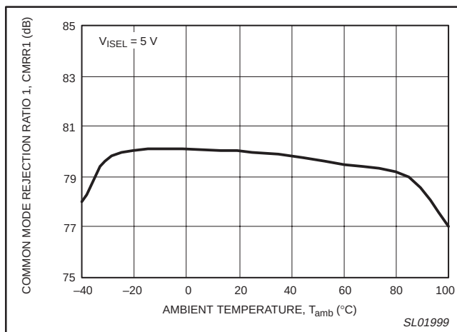
Figure 24. Common mode rejection ratio 1 versus ambient temperature.
