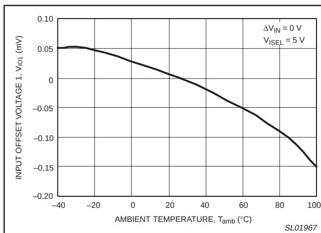
Figure 8. Input offset voltage 1 versus ambient temperature.
