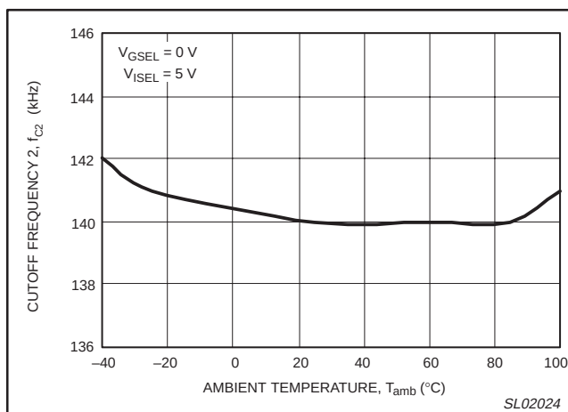
Figure 30. Cutoff frequency 2 versus ambient temperature.
