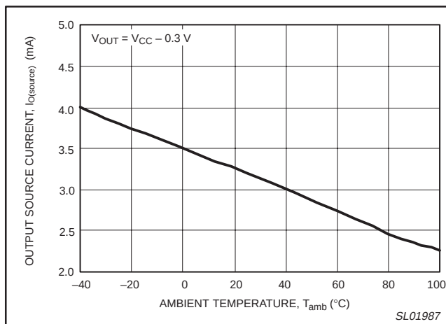
Figure 16. Output source current versus ambient temperature.
