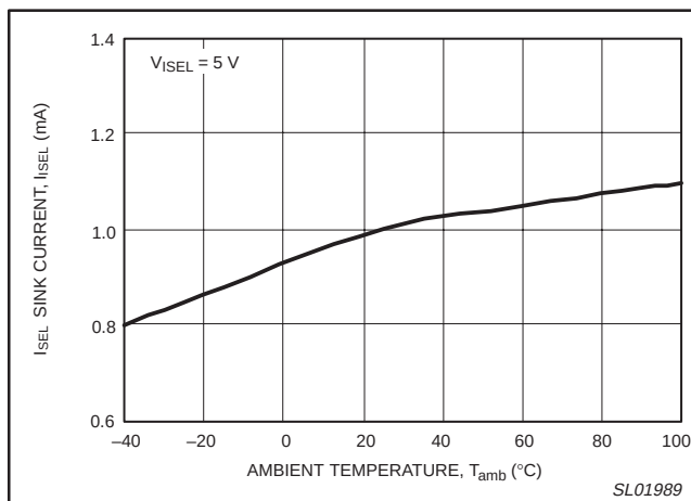
Figure 18. I_{SEL} sink current versus ambient temperature.
