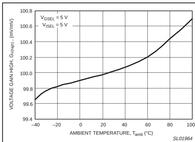
Figure 4. Voltage Gain 1 (HIGH) versus ambient temperature.
