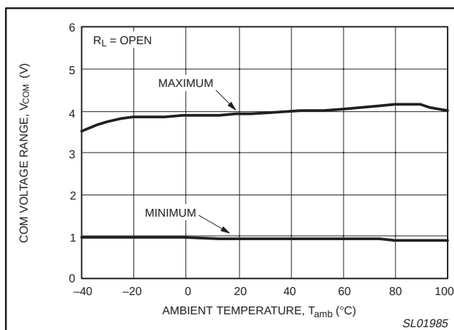
Figure 14. COM voltage range versus ambient temperature.
