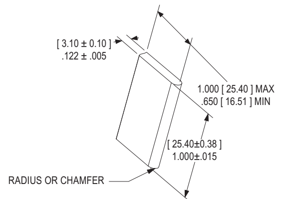
Mating Blade
