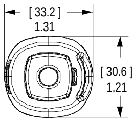
Front Without Strain Relief
