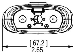
Front With Strain Relief
