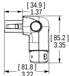
Side With Strain Relief
