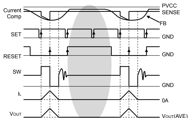
Fig.21 SLLM™ Not switching timing chart
