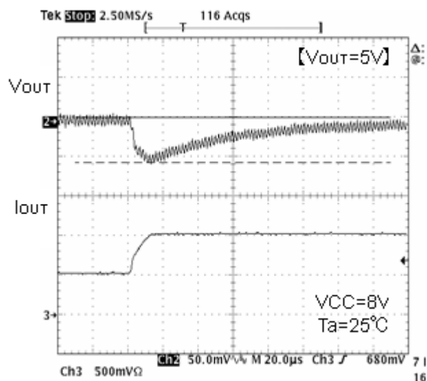
Fig.17 Transient response I_o=0.5\text{A} \rightarrow 1\text{A}(10\mu\text{s})
