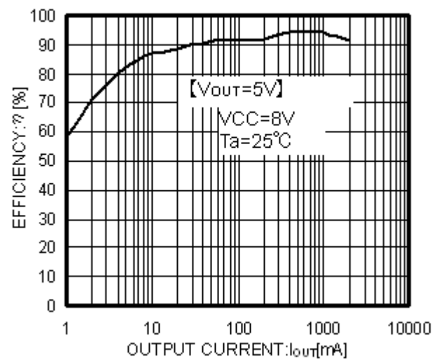
Fig.8 Efficiency
