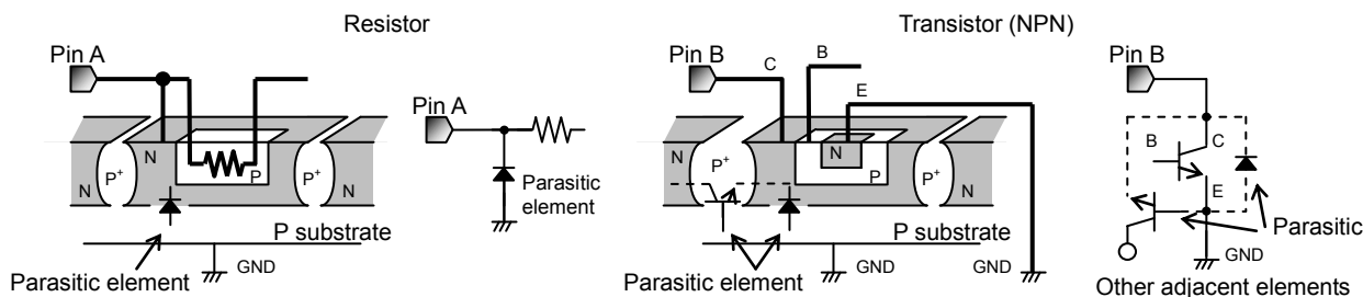
Fig.38 Simplified structure of monoristic IC
