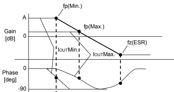
Fig.31 Open loop gain characteristics
