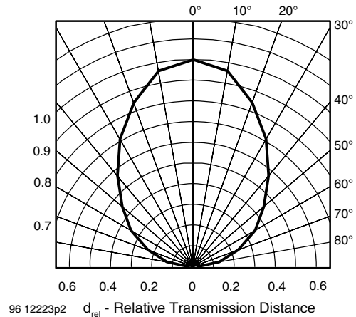
Fig. 12 - Horizontal Directivity
