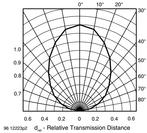
Fig. 12 - Horizontal Directivity
