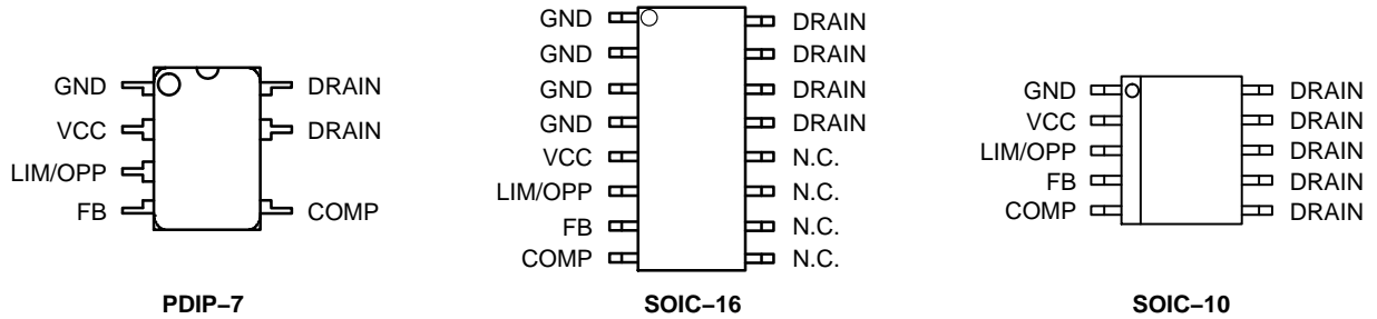
Figure 1. Pin Connections
