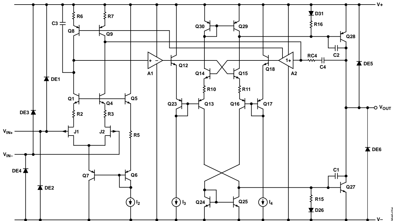
Figure 56. Simplified Schematic
