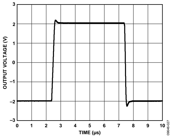
Figure 33. Large Signal Transient Response, V_{SY} = \pm 5\text{ V} , A_V = +1 , R_L = 2\text{ k}\Omega , C_L = 100\text{ pF}
