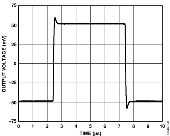
Figure 34. Small Signal Transient Response, V_{SY} = \pm 5\text{ V} , A_V = +1 , R_L = 2\text{ k}\Omega , C_L = 100\text{ pF}
