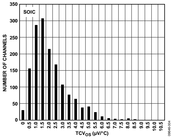
Figure 9. Input Offset Voltage Drift (TCV OS ) Distribution, V SY = ±5 V
