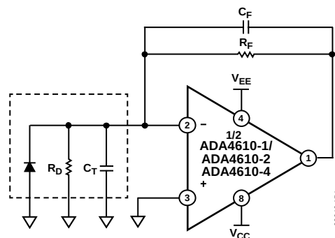
Figure 58. Equivalent Preamplifier Photodiode Circuit
