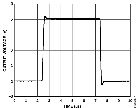
Figure 33. Large Signal Transient Response, V_{SV} = \pm 5\text{ V} , A_V = +1 , R_L = 2\text{ k}\Omega , C_L = 100\text{ pF}
