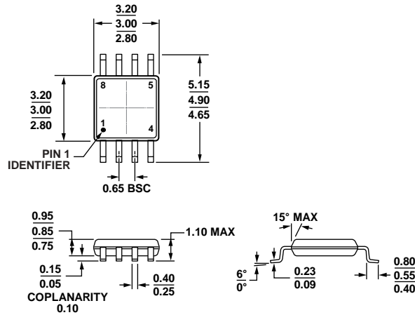
COMPLIANT TO JEDEC STANDARDS MO-187-AA Figure 61. 8-Lead Mini Small Outline Package [MSOP] (RM-8)
