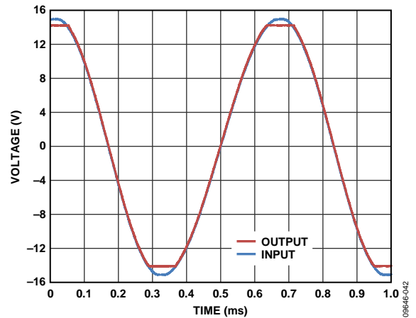
Figure 47. No Phase Reversal, V_{SY} = \pm 15 V , A_V = +1 , R_L = 2 k\Omega , C_L = 100 pF
