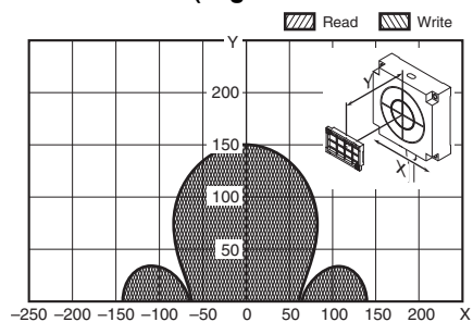
V680-HS63 (with Metal on Back Surface) & V680S-D2KF68M (Metal on back: Steel) (Tag direction: Horizontal) V680S-D2KF68M (Metal on back: Steel) (Tag direction: Vertical)
