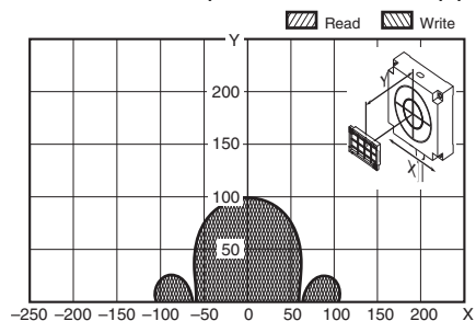
V680-HS65 (with Metal on Back Surface) & V680S-D2KF68M (Metal on back: Steel) (Tag direction: Horizontal) V680S-D2KF68M (Metal on back: Steel) (Tag direction: Vertical)
