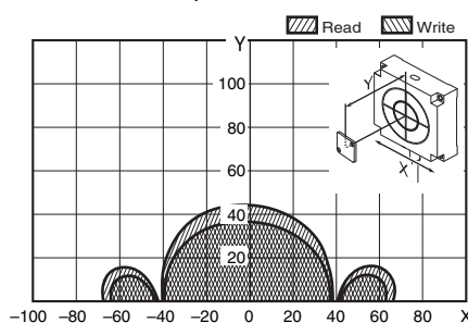
V680-HS65 (mounted on metallic material) & V680-D1KP66MT (mounted on metallic surface: steel)
