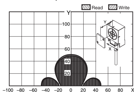
V680-H01-V2 (mounted on non-metallic material) & V680-D1KP66T (mounted on non-metallic material)
