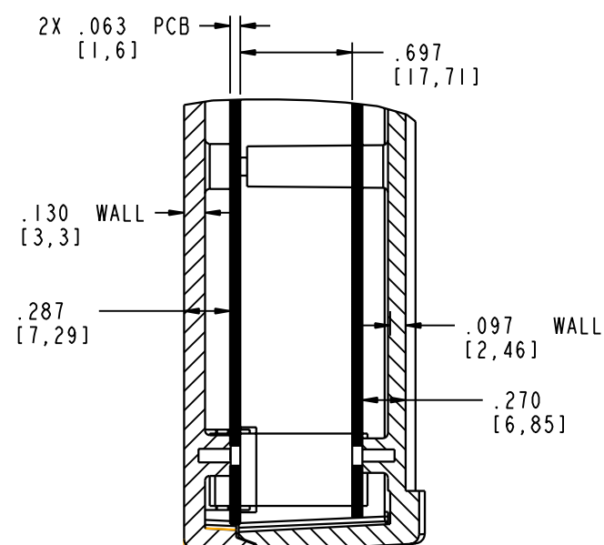
SECTION C-C SCALE 2.000
