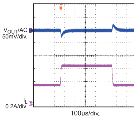
Load Transient Response I_{OUT} = 0.3A-0.6A , C_{FF}=150pF
