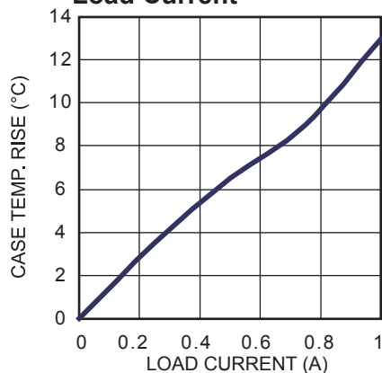
Case Temp. vs. Load Current
