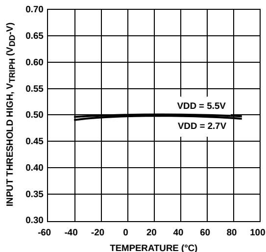
FIGURE 5. V_{TRIP_H} VOLTAGE
