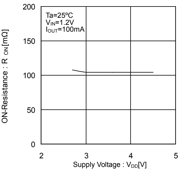
Figure 7. ON-Resistance vs Supply Voltage (BD6528HFV)
