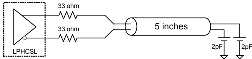
LP HCSL output test conditions
