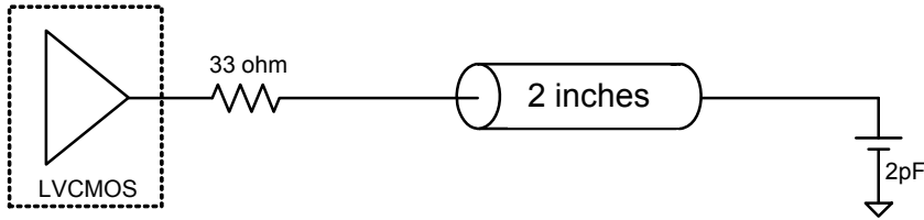
LVC MOS output test conditions
