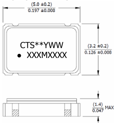
PACKAGE DRAWING
