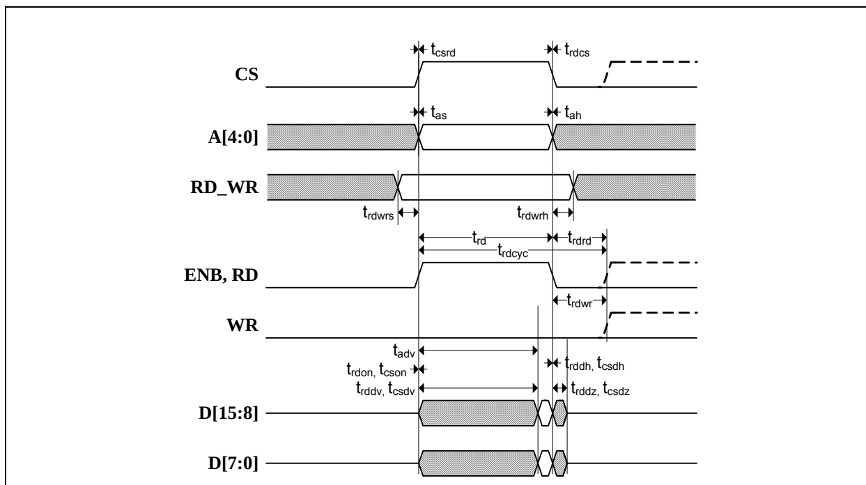
FIGURE 9-36: INDEXED ADDRESSING READ CYCLE TIMING
