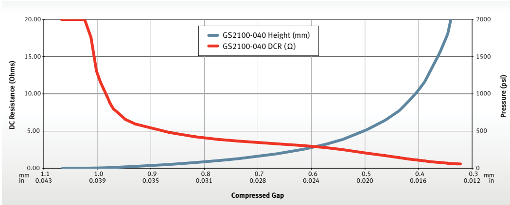
FIGURE 5: GS2100-040 FORCE DISPLACEMENT RESISTANCE (testing with 5 x 5 mm grounding pads)
