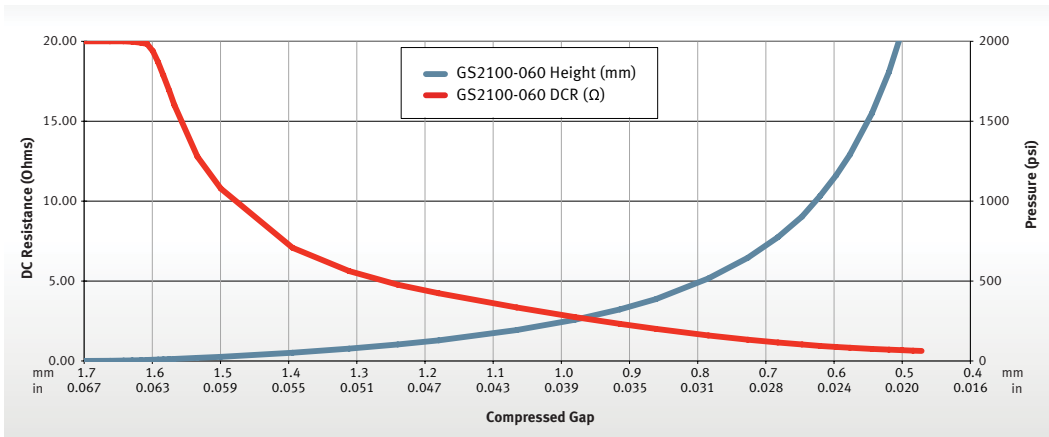
FIGURE 6: GS2100-060 FORCE DISPLACEMENT RESISTANCE (testing with 5 x 5 mm grounding pads)
