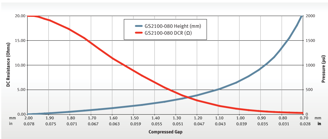
FIGURE 7: GS2100-080 FORCE DISPLACEMENT RESISTANCE (testing with 5 x 5 mm grounding pads)
