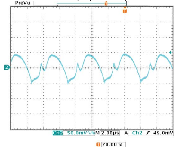
Output Ripple and Noise ( V_{in}=48V , V_{out}=nom , I_{out}=10A , C_{out}=1F \parallel 10\mu F \parallel 4700\mu F , T_a=+25^\circ C , ScopeBW=20Mhz)
