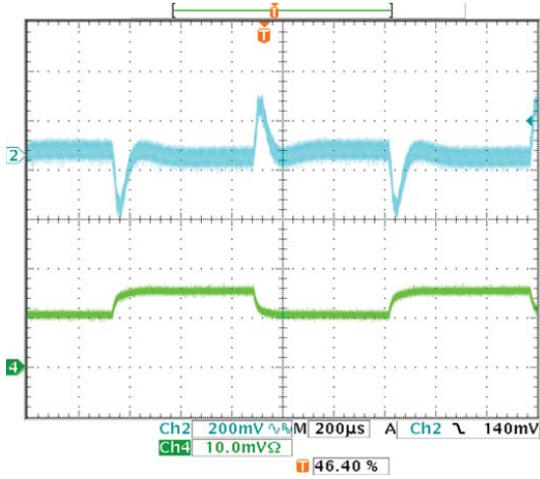
Output Ripple and Noise (Vin=48V, Vout=nom, Iout=0A, Cout=1F || 10μF, Ta=+25°C, ScopeBW=20Mhz)
