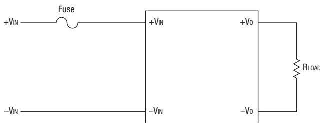
Figure 2. Input Fusing
