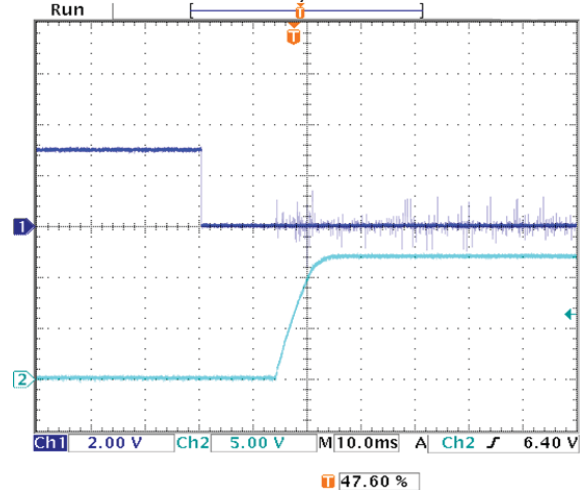
On/Off Enable Delay (Vin=48V, Iout=10A, Cout=4700µF, Ta=+25°C) Trace1=Enable, Trace2=Vout.
