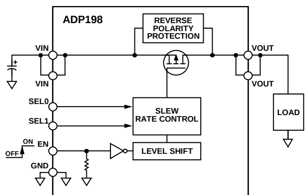
Figure 2. LFCSP
