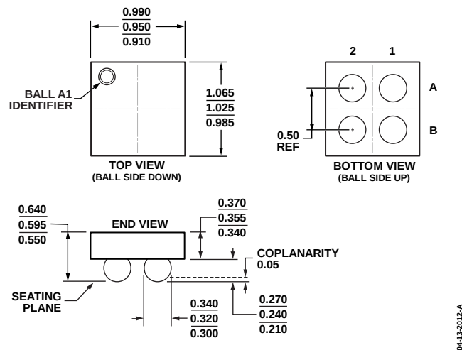
Figure 33. 4-Ball Wafer Level Chip Scale Package [WL CSP] (CB-4-4) Dimensions shown in millimeters
