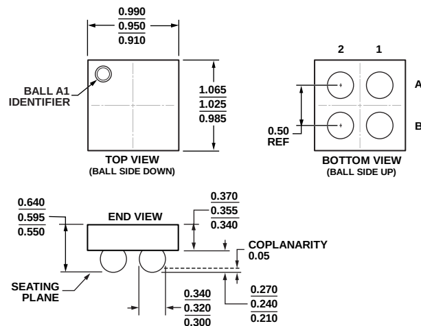
Figure 33. 4-Ball Wafer Level Chip Scale Package [WLCSP] (CB-4-4)
