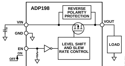
Figure 1. WLCSP
