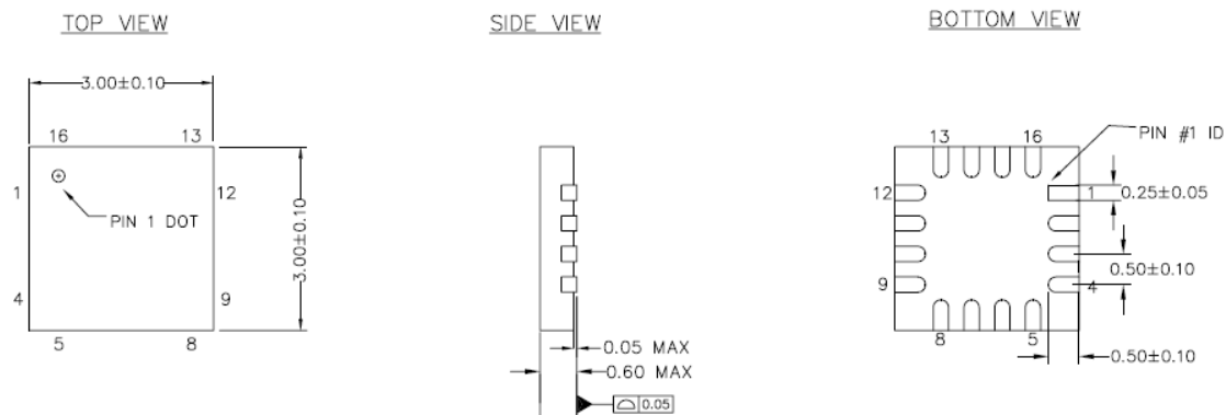
Figure 20. 16-pin QFN (No E-Pad) (3 × 3 × 0.6 mm) LG16A (Sawn) Package Outline, 001-09116
