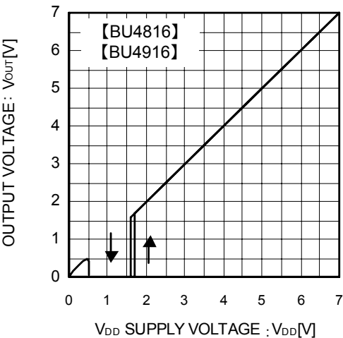
Fig.6 I/O Characteristics
