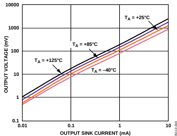
Figure 12. Output Voltage vs. Output Sink Current ( I_{sink} = 500\text{ mA} )
