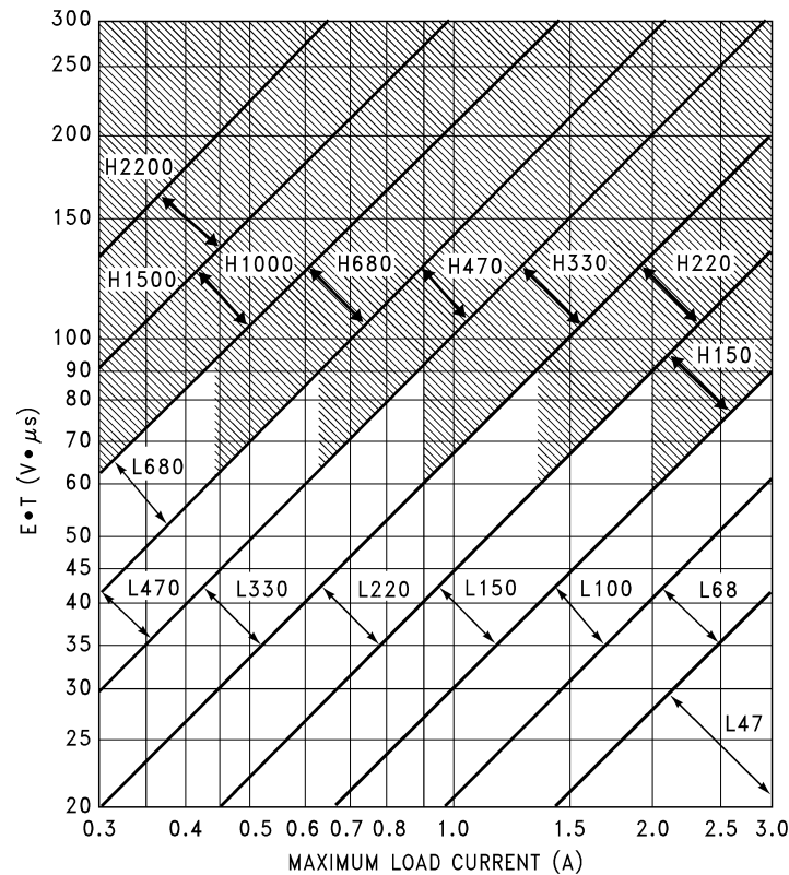
Figure 27. LM2576(HV)-ADJ
