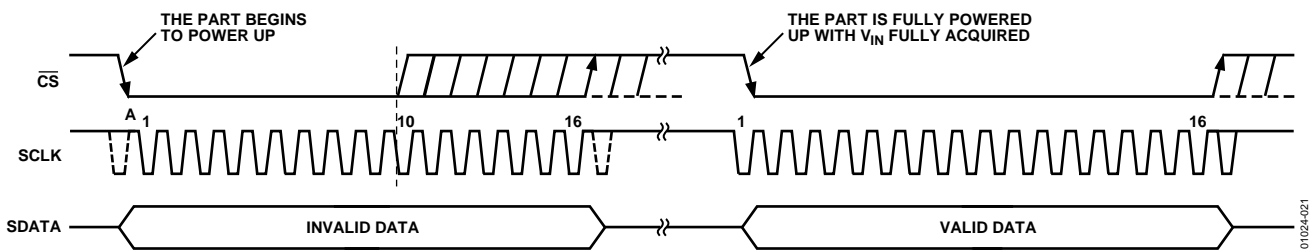
Figure 21. Exiting Power-Down Mode
